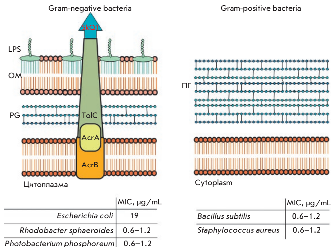
Fig. 1. Schematic of the bacterial cell wall (LPS – lipopolysaccharides, OM – outer membrane, PG – peptidoglycan layer) and the antibacterial effect of SkQ1 against gram-positive and gram-negative bacteria. The sensitivity of gram-negative bacteria to SkQ1 depends on the structure of the protein components of the AcrAB-TolC pump
